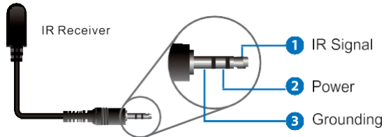
IR RECEIVER
